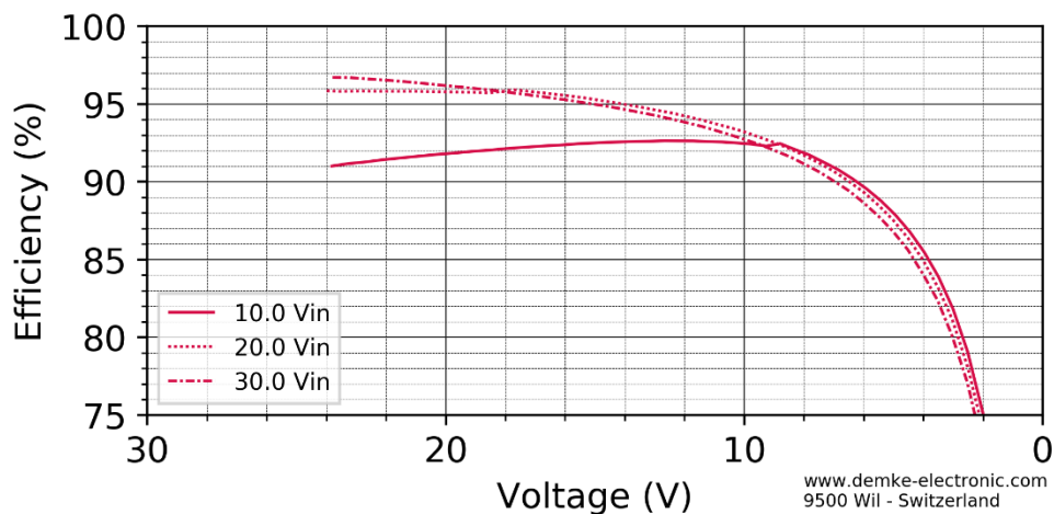
Figure 3 Efficiency in the constant current range of the DC-Transformer 257LE-24-SD
