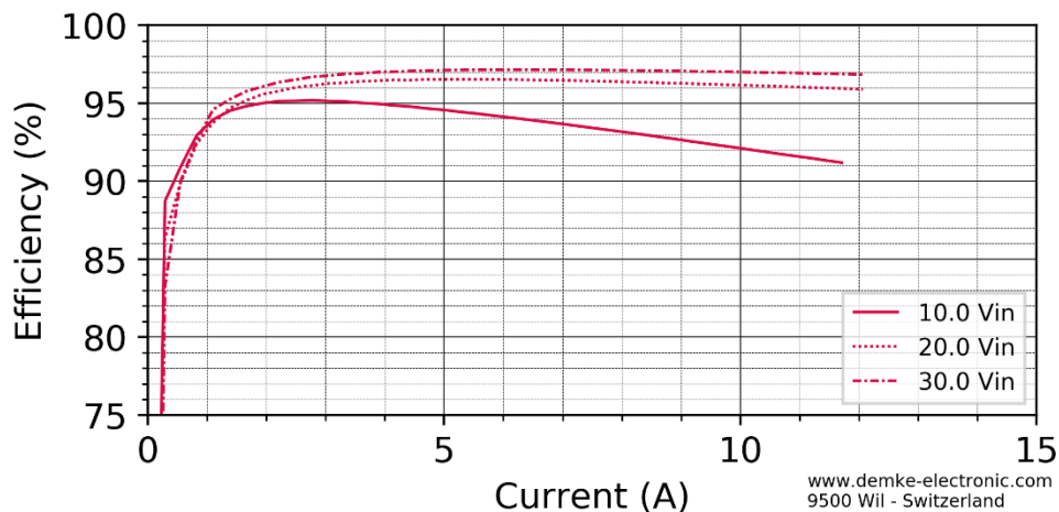
Figure 2 Efficiency in the constant voltage range of the DC-Transformer 257LE-24-SD
