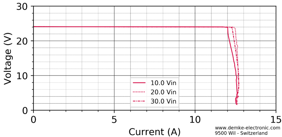
Figure 1 Voltage against current of the DC-Transformer 257LE-24-SD
