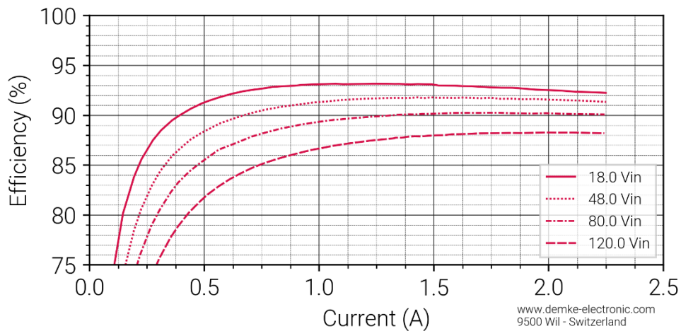
Figure 2 Efficiency in the constant voltage range of the DC-Transformer 344W-24-SD
