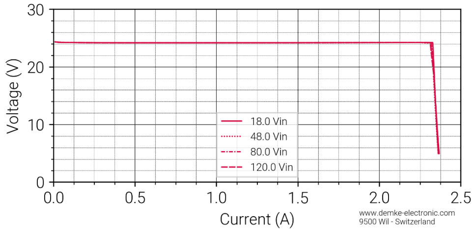
Figure 1 Voltage against current of the DC-Transformer 344W-24-SD
