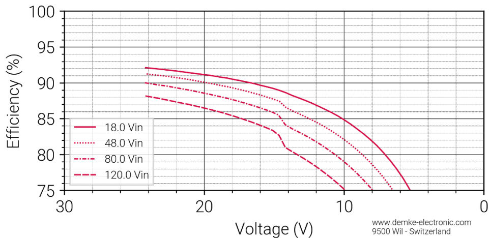
Figure 3 Efficiency in the constant current range of the DC-Transformer 344W-24-SD
