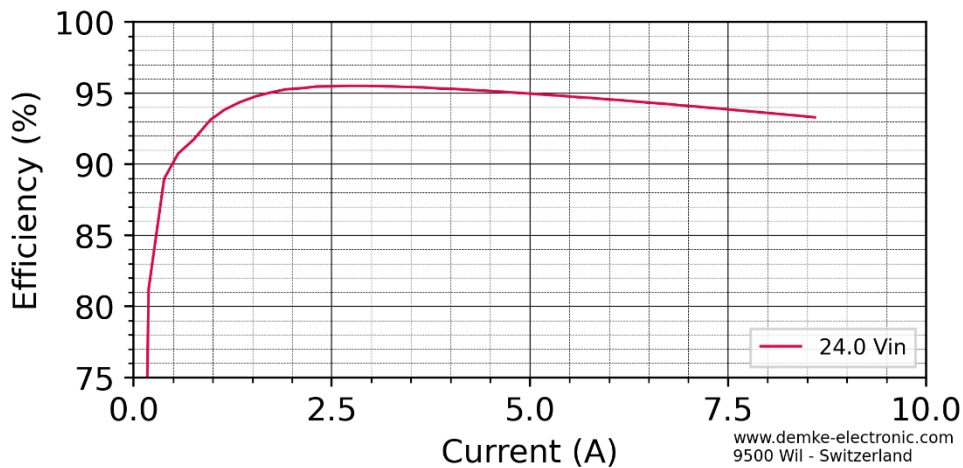
Figure 2 Efficiency in the constant voltage range of the DC-Transformer 739-92-SD
