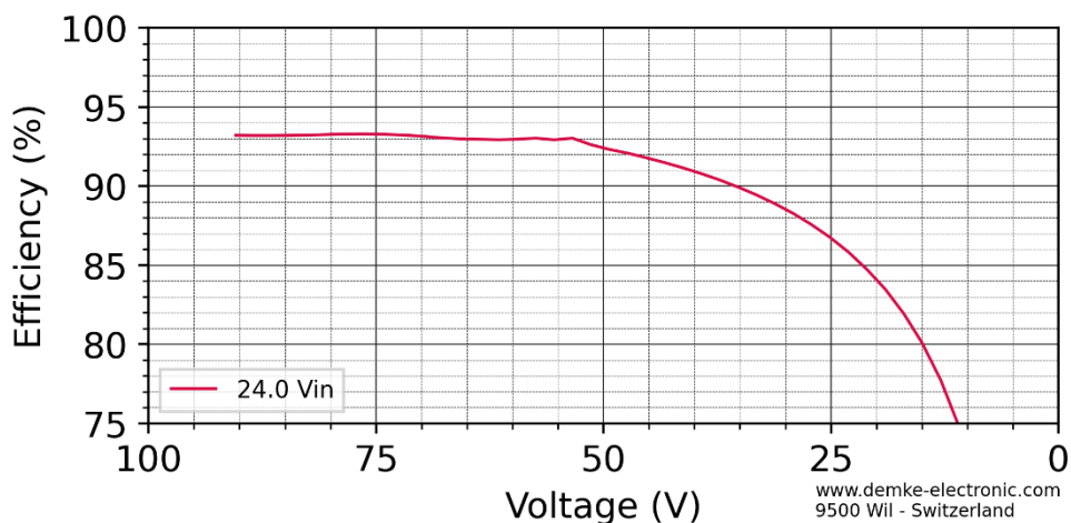
Figure 3 Efficiency in the constant current range of the DC-Transformer 739-92-SD
