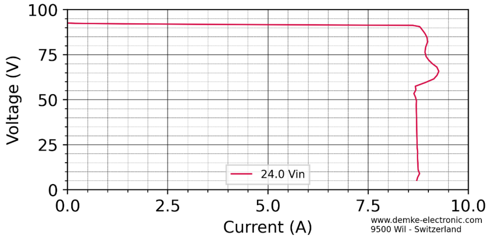
Figure 1 Voltage against current of the DC-Transformer 739-92-SD
