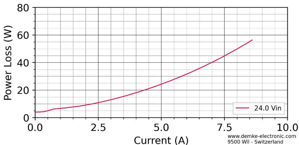
Figure 5: Power Loss over voltage of the DC-Transformer 739-92-SD
