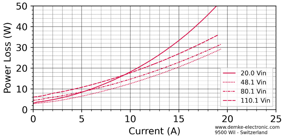
Figure 4: Power Loss over current of the DC-Transformer 755-24-SD
