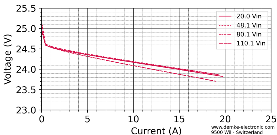
Figure 6: Voltage in CV-mode of the DC-Transformer 755-24-SD
