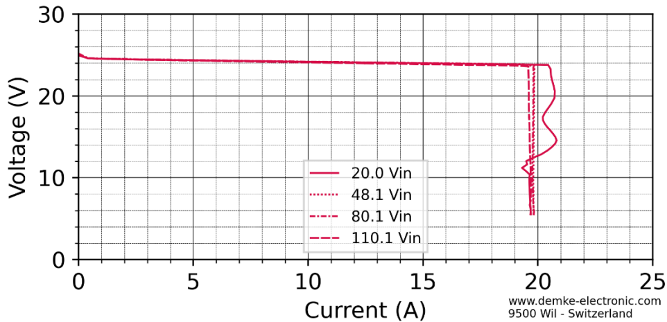
Figure 1 Voltage against current of the DC-Transformer 755-24-SD
