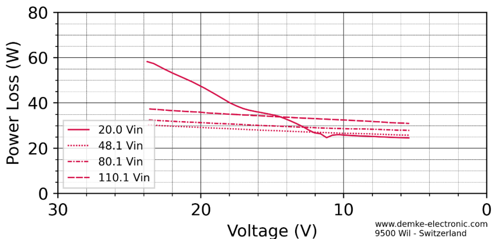
Figure 5: Power Loss over voltage of the DC-Transformer 755-24-SD
