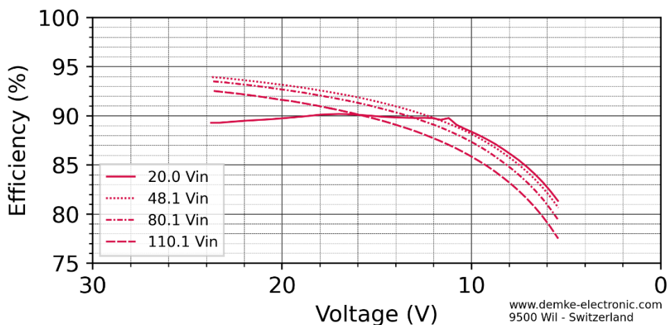
Figure 3 Efficiency in the constant current range of the DC-Transformer 755-24-SD
