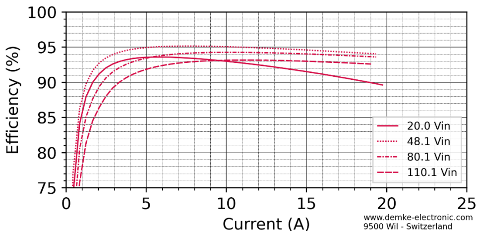
Figure 2 Efficiency in the constant voltage range of the DC-Transformer 755-24-SD
