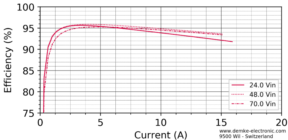
Figure 2 Efficiency in the constant voltage range of the DC-Transformer 757-48-SD
