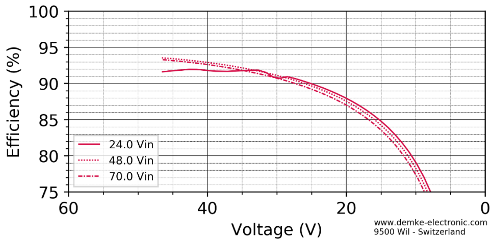
Figure 3 Efficiency in the constant current range of the DC-Transformer 757-48-SD
