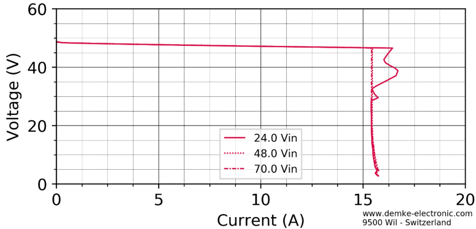
Figure 1 Voltage against current of the DC-Transformer 757-48-SD
