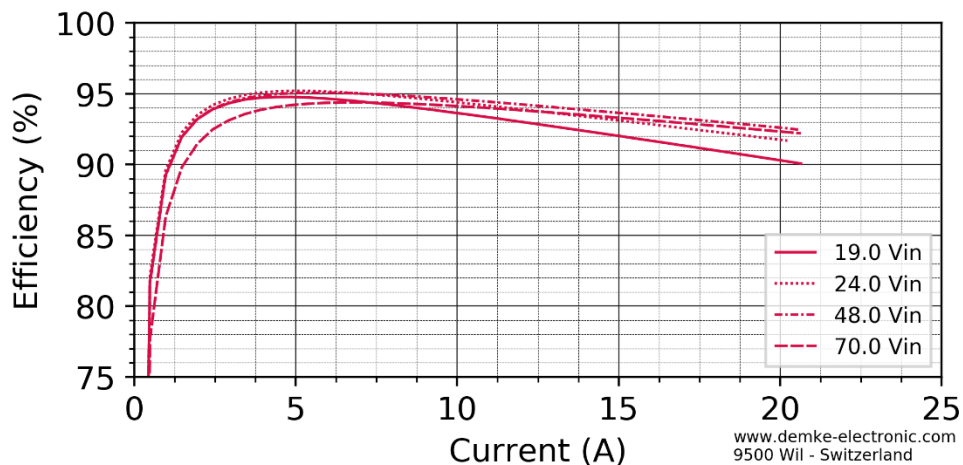
Figure 2 Efficiency in the constant voltage range of the DC-Transformer 757-27-SD
