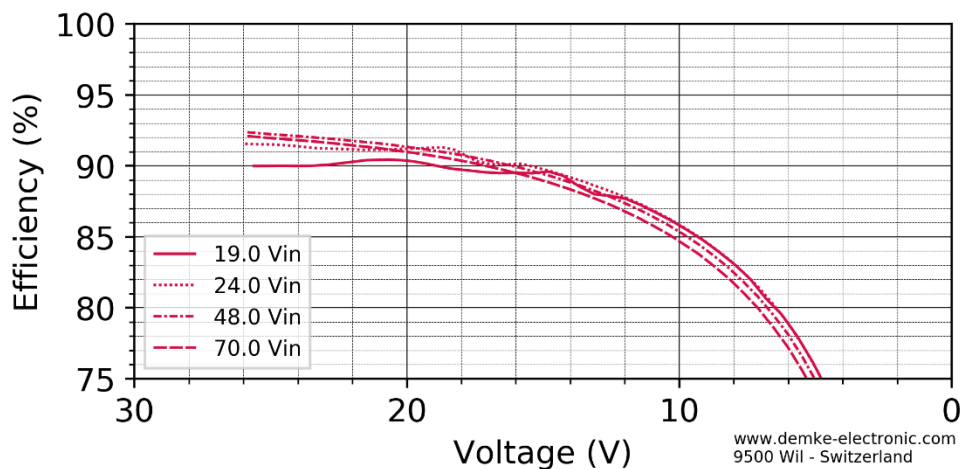
Figure 3 Efficiency in the constant current range of the DC-Transformer 757-27-SD
