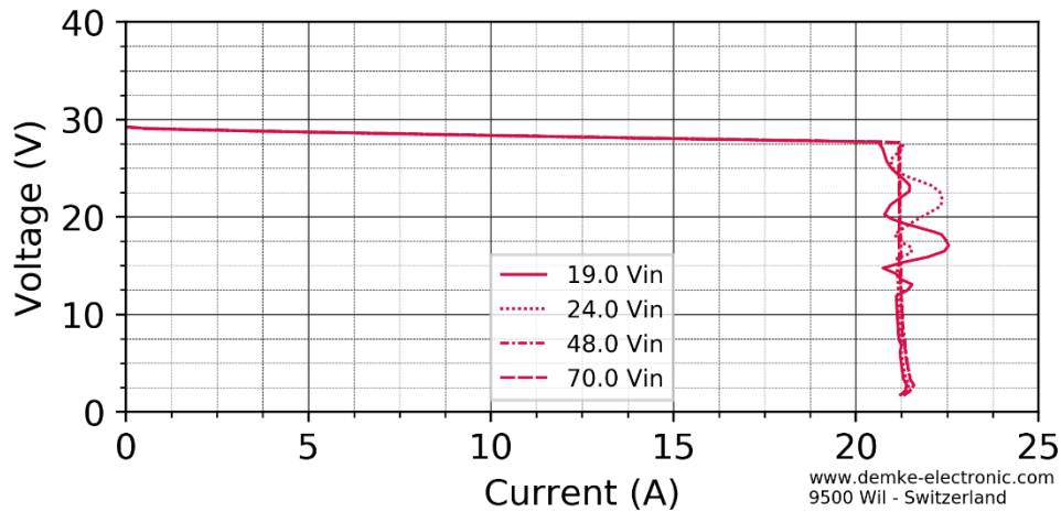
Figure 4 Voltage against current of the DC-Transformer 757-27-SD in SH mode
