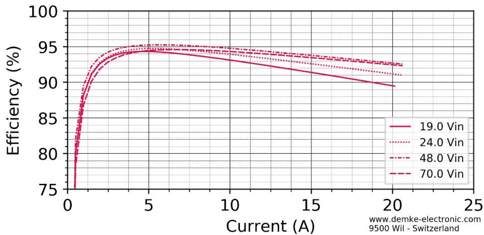
Figure 5 Efficiency in the constant voltage range of the DC-Transformer 757-27-SD in SH mode
