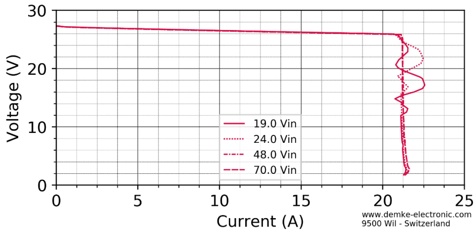
Figure 1 Voltage against current of the DC-Transformer 757-27-SD
