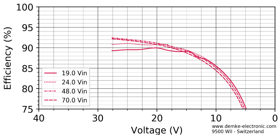
Figure 6 Efficiency in the constant current range of the DC-Transformer 757-27-SD in SH mode
